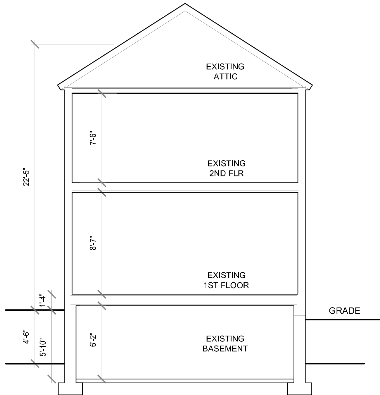
BLG SECTION @ COUCH HOUSE 1/8" = 1'-0"
