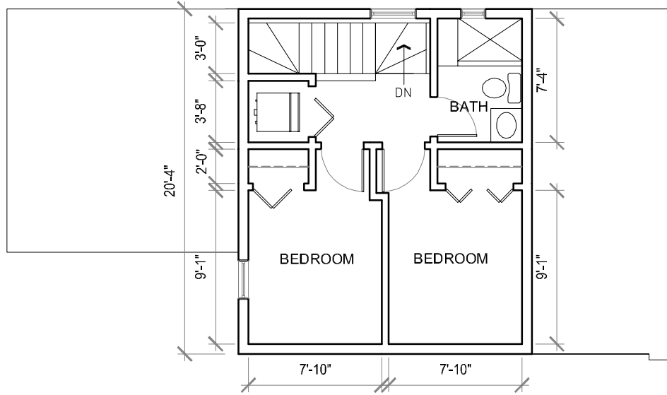
2ND FLR PLAN
